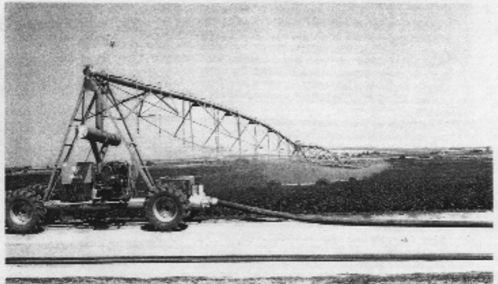
Linear move system
